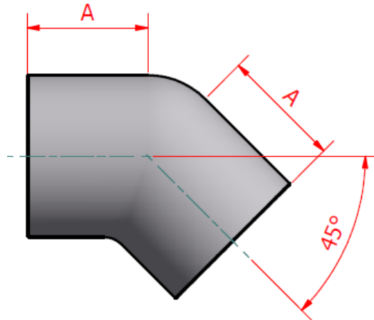
45 degree female elbow
