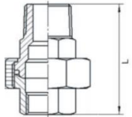
Male/female socket union
