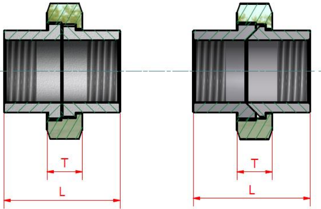
Female socket union
