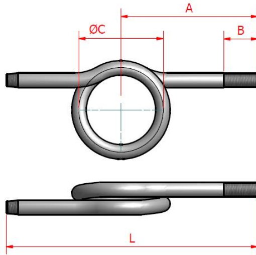
Ring syphon
