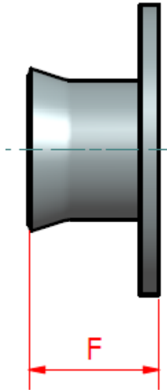
Flanged adaptor
